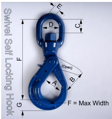
Swivel self locking hook
