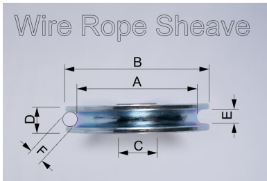
Wire rope sheave
