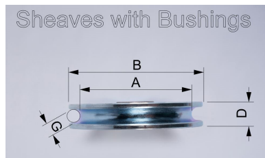
sheave with bushing2
