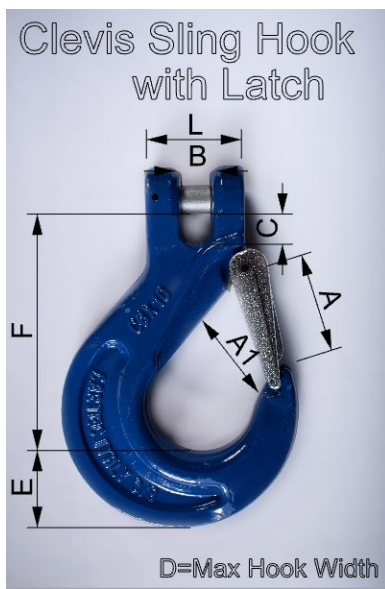
clevis sling hook w latch
