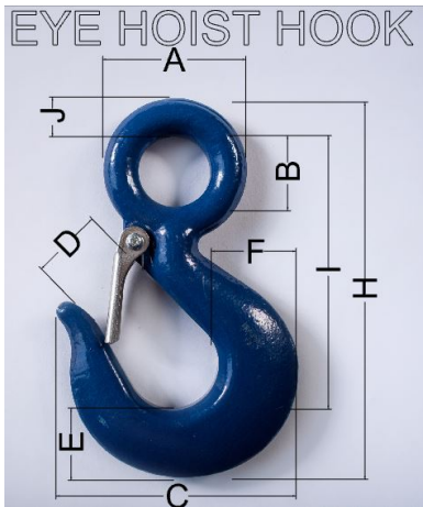
eye hoist hook
